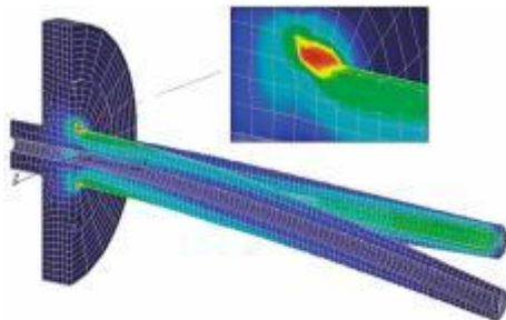
FEA representation of a thermowell in flow with stress at the tip and root
